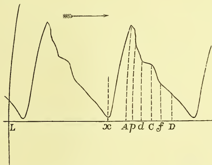
FIG. 44. PULSE TRACING FROM THE RADIAL ARTERY OF MAN.
